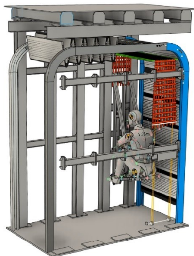
Schematic view of SHELTER (Structural Hyper-resisting Element for Life Threatening Earthquake Risk) with a safety chair and a dummy.
