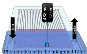
Photodiode integration
