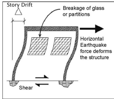
Figure 5. Non-structural damage due to building deformation [6].
