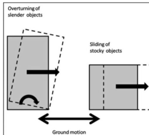
Figure 4. Sliding and overturning due to inertial forces [6].
