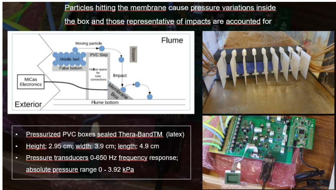
Figure 2. In-house pressure-based bedload discharge meter.
