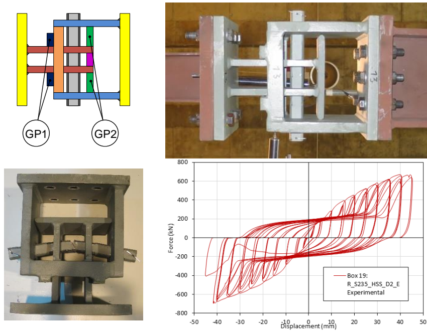
Figure 1. DRBRC – Device developed and tested in Instituto Superior Técnico.
