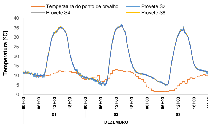
Figure 2. Surface temperatures and dew points of specimens exposed at LNEC aging site during December 2020.
