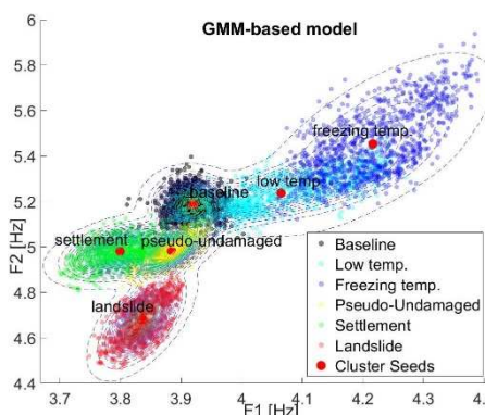
FE model of Z-24 Bridge (left); Classification based on hybrid data and Gaussian Mixture Models (right).
