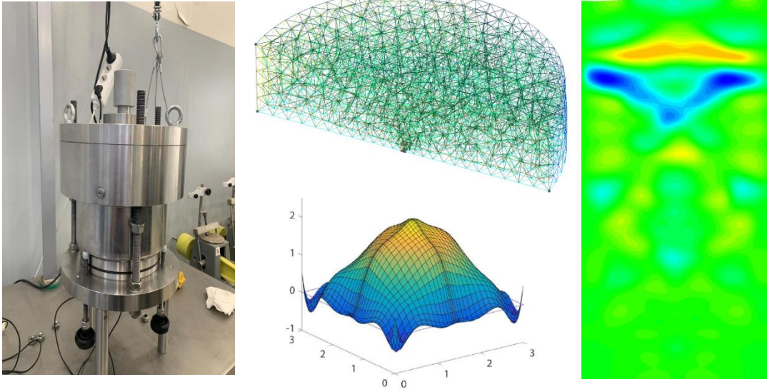
Figure 1. a) Innovative Rowe cell fitted with bender elements; b) Sample mesh for the computational modelling of a soil sample in the modified Rowe cell; c) Particular solution field in a heat propagation problem modelled with hybrid-Trefftz finite elements; d) Propagation of a shear wave through a saturated soil.
