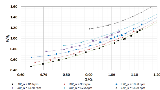
Figure 5. Experimental results for different rotational speeds.
