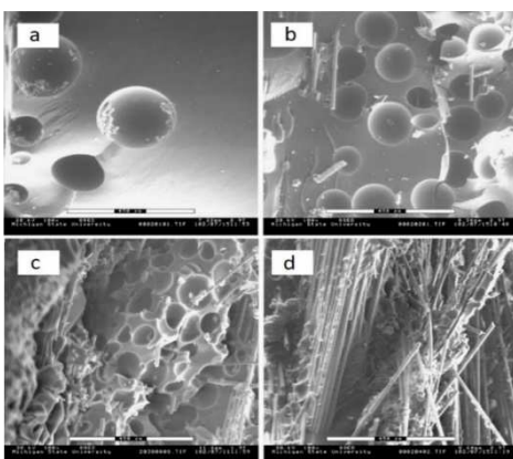
ESEM micrographs of glass reinforced biobased polyurethanes: (a) no fiber, (b) 15 wt%, (c) 30 wt% and (d) 50 wt%, Dwan'Isa et. al. (2004).
