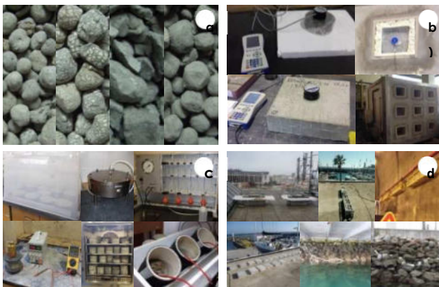
Overview of the experimental campaign: a) different types of LWA; b) thermal characterization; c) durability characterization; d) different environmental exposure conditions.
